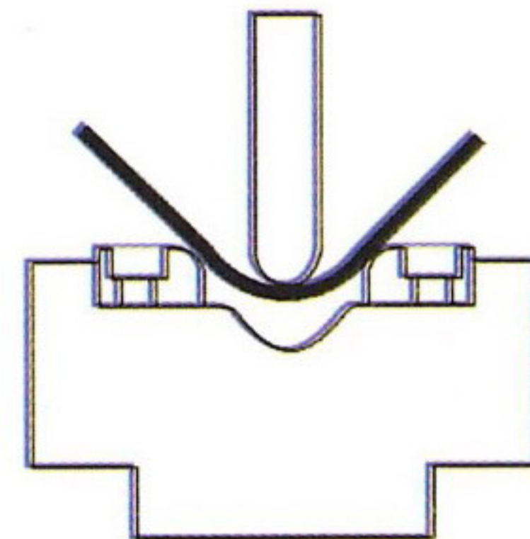
Curling dies
