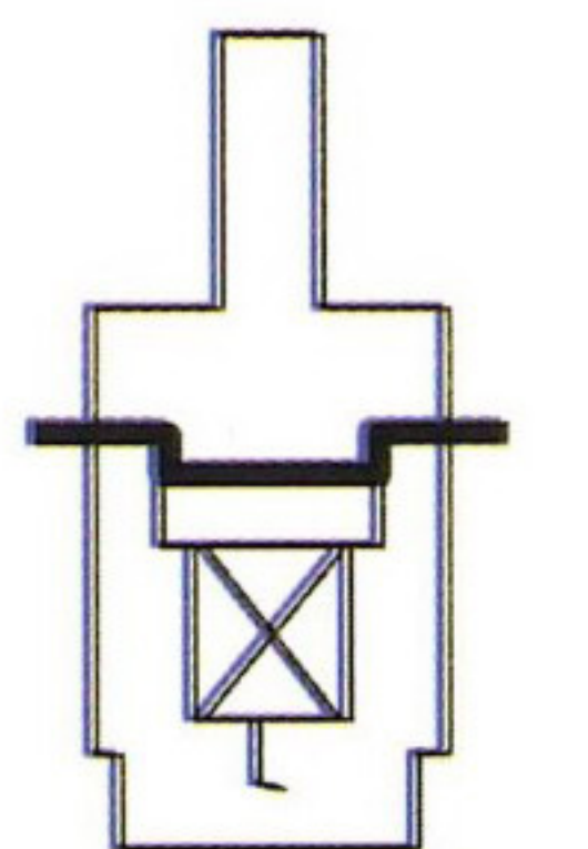
Corrugating dies
